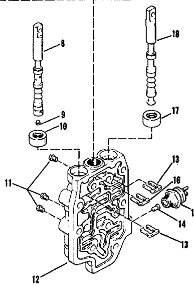
HYDRAULIC DECLUTCH
