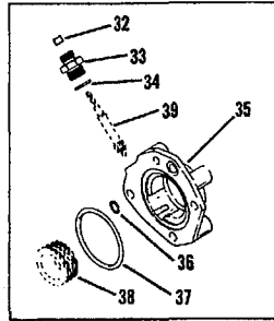
PARKING BRAKE WITH SPEED GEAR
