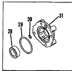
PARKING BRAKE LESS SPEED GEAR
